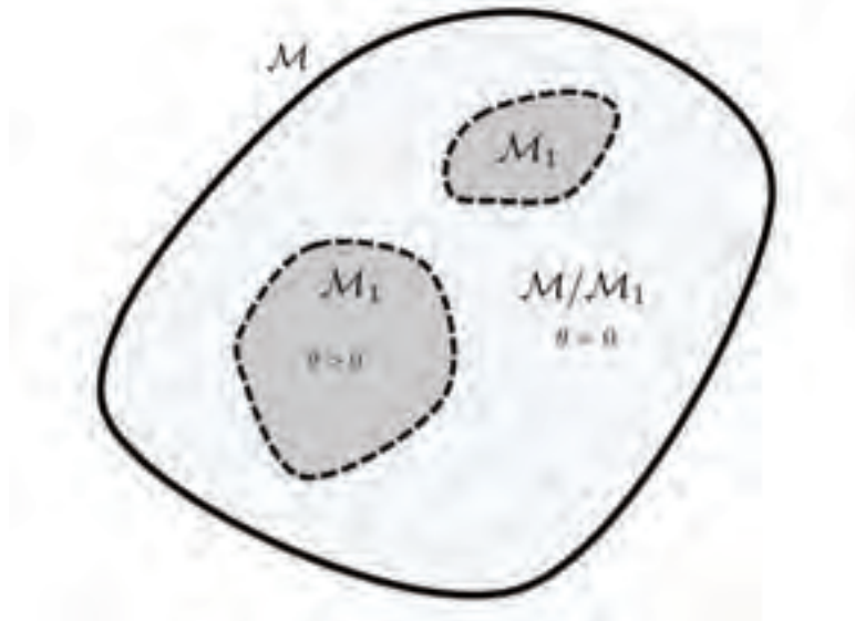
Figure 3: Under H_1 , there exist nonempty rejection regions \mathcal{M}_1 where the signal is significant, i.e. \theta > 0 . The power is computed with respect to these rejection regions.
